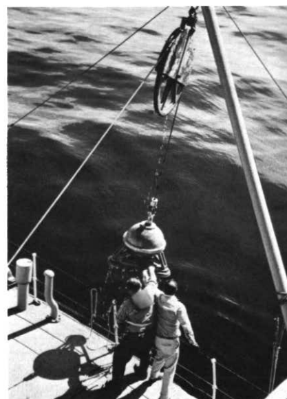
Figure 6 A La Coste and Romberg underwater gravity meter is hauled aboard after an observation on the sea-floor.
