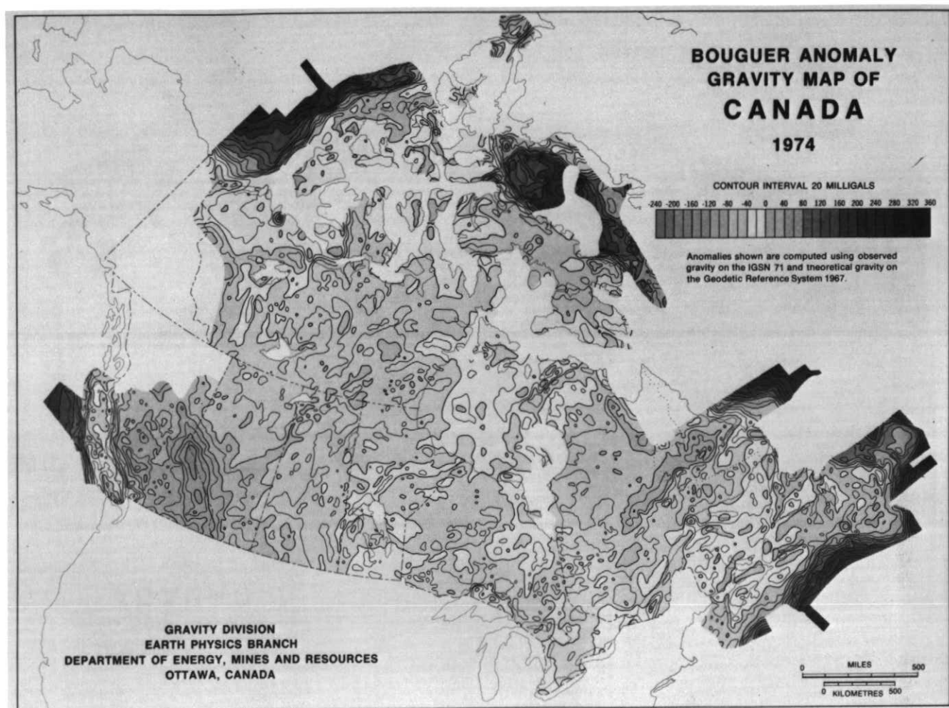
Figure 4 Gravity Map of Canada.
