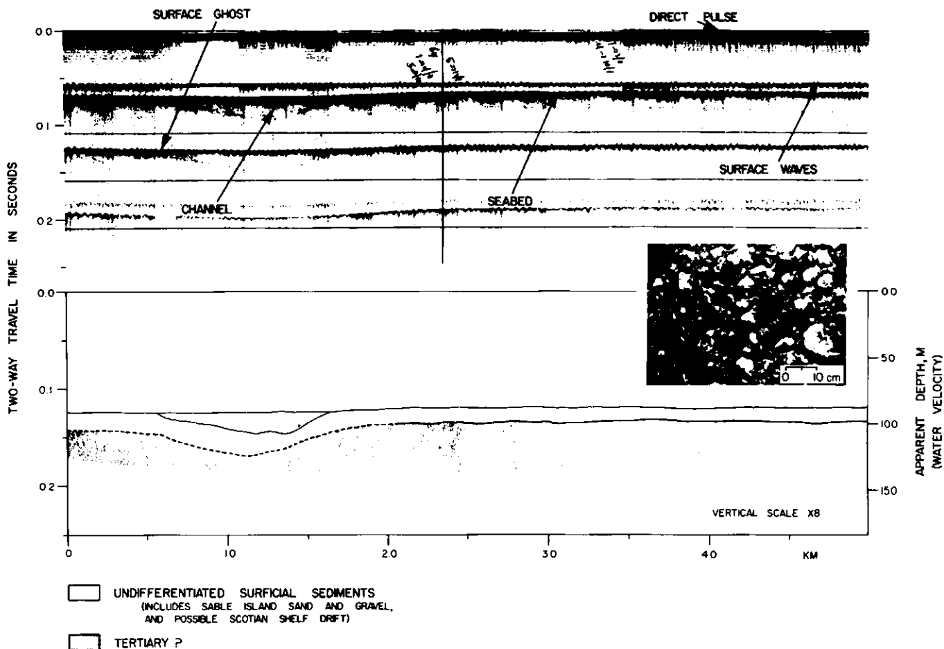
Figure 6 Seismic profile across the gravel facies (see inset) of the Sable Island sand and gravel on Emerald Bank between fixes 63 and 65 of Figure 4.
