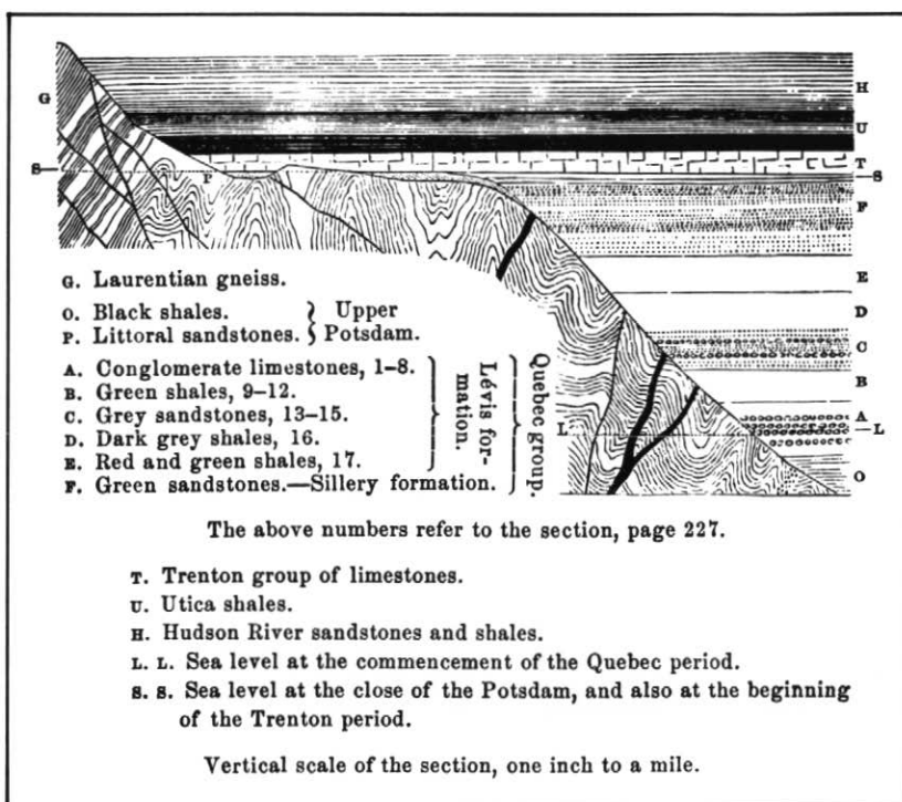
Figure 2 Disposition of the Quebec Group before thrusting. (from Logan, 1863a).
