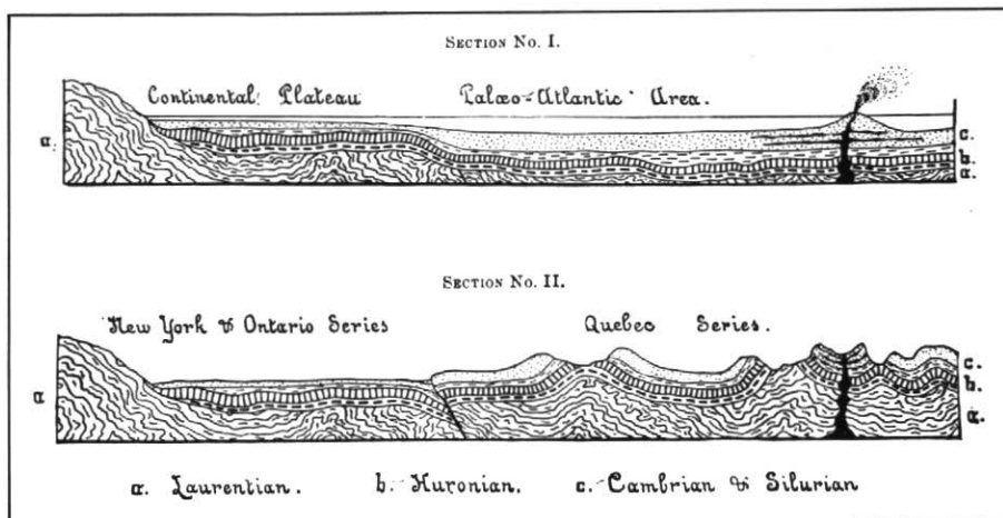
Figure 3 Logan's concept of the ancient margin of North America before deformation (section 1) and after (section 2). According to Dawson, in Harrington, 1883.
