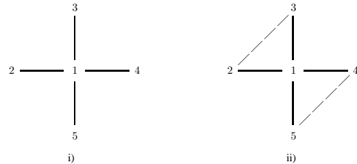
Figure 3. (i) Case 1b; (ii) Patching inducing disconnection of A' in case 1b.
