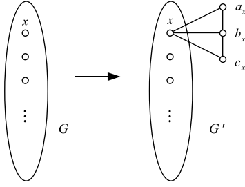
Fig. 5. Construction of G' from G . To each vertex x of G , we connect the three vertices of a path a_x b_x c_x .
