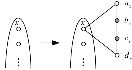
Fig. 2. For any vertex x of G which is not in D , the vertices b_x and c_x belong to D_t .
