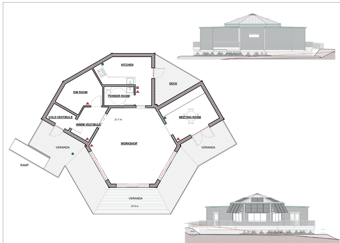
FIG. 9. SUBSEQUENT DRAFT DESIGN SHOWING THE FLOOR PLAN AND PROFILE OF THE BUILDING WHEN OPTIMIZED FOR ENERGY EFFICIENCY. | PI/KHS AND SAIT GBAC BUILDING PLANS AND BLUEPRINTS. ON FILE AT PI/KHS ARCHIVES.
