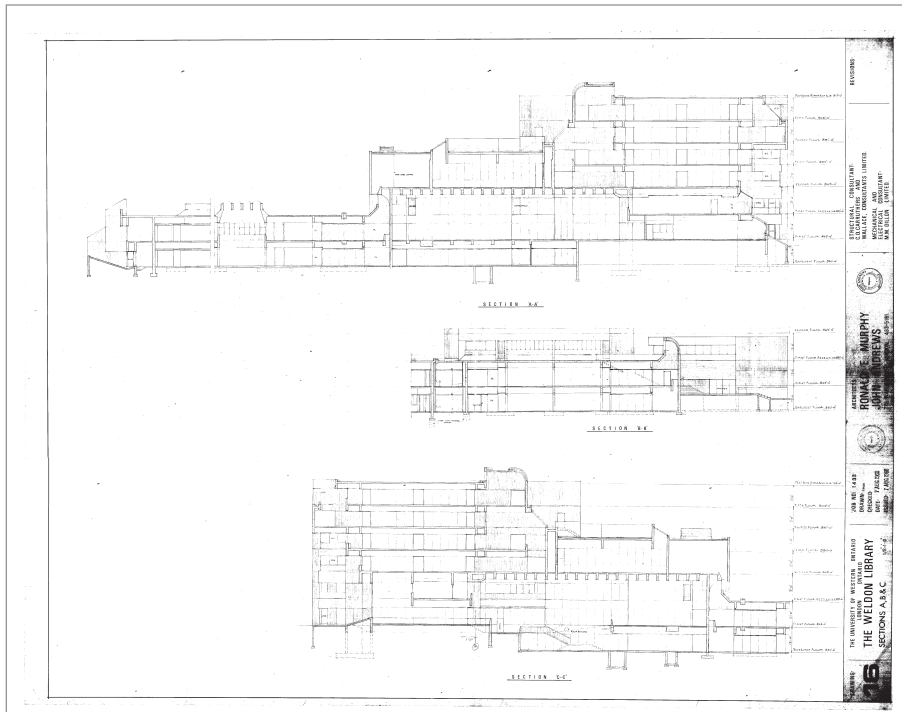
FIG. 5. THE MULTI-STOREY "MEETING PLACE" AS A CENTRAL SPACE OF CIRCULATION AND COMMUNICATION IS EVIDENT IN BUILDING SECTIONS A AND C, DRAWING A16, THE WELDON LIBRARY (RONALD E. MURPHY / JOHN ANDREWS, 1968), THE UNIVERSITY OF WESTERN ONTARIO, LONDON. | FACILITIES MANAGEMENT, WESTERN UNIVERSITY.
