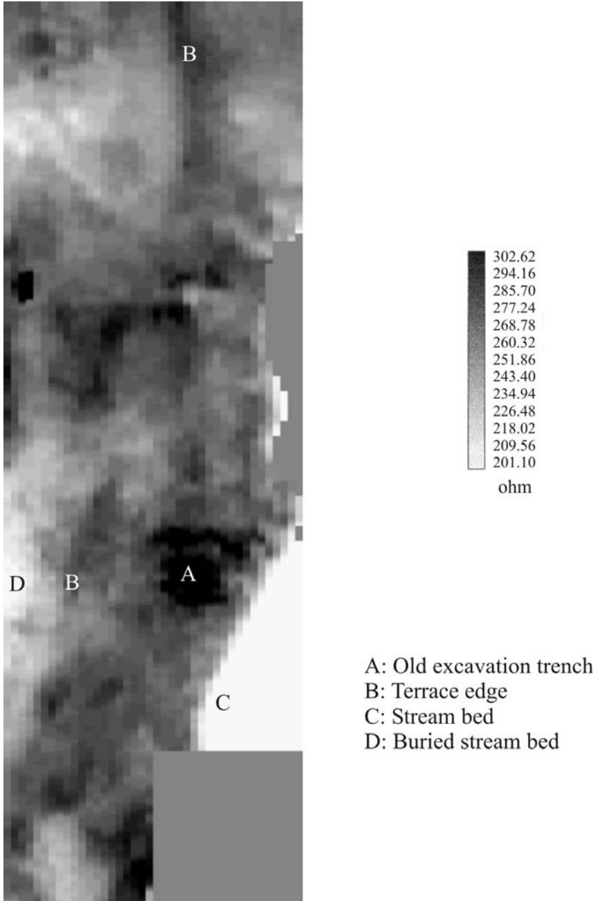
Figure 3. Results of the resistivity survey.
