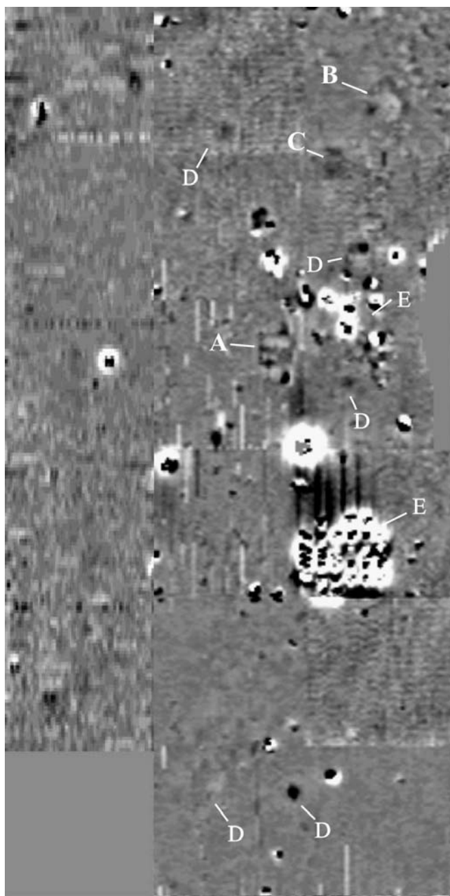
Figure 4. Results of the close interval magnetometer survey. Note: the western six grids are added from the broad interval survey.
