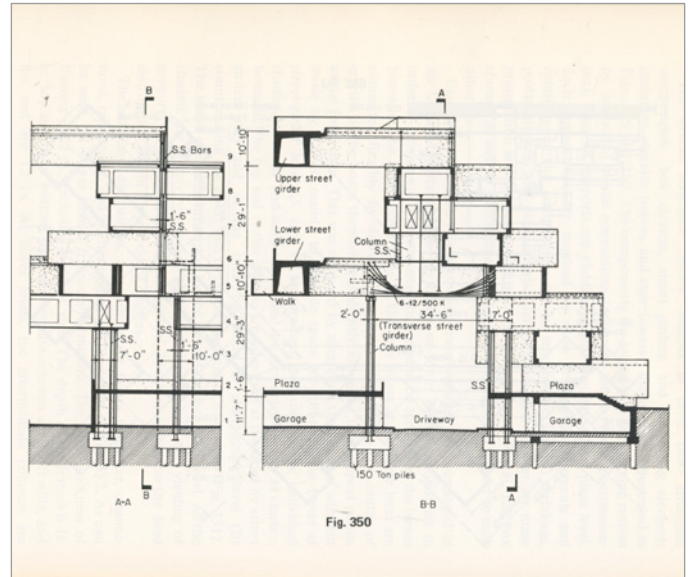
FIG. 17. SECTIONS FOR BOX CLUSTERS, STREET GIRDERS, AND COLUMNS, AUGUST KOMENDANT, 1965. | AUGUST KOMENDANT, CONTEMPORARY CONCRETE STRUCTURES , HUNTINGTON, NY, R.E. KRIEGER, 1977, P. 538. COURTESY: THE ARCHITECTURAL ARCHIVES, UNIVERSITY OF PENNSYLVANIA.
