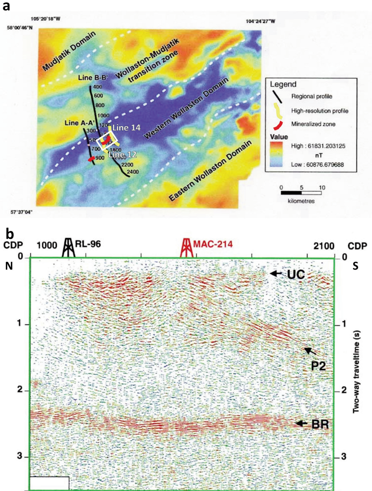
Figure 29. a) Total field magnetic map of the McArthur River study area with lithotectonic domains shown. Seismic lines are identified. Numbers are common-depth-point (CDP) locations. The white rectangle outlines the location of the low-fold 3-D acquisition program. b) Enlarged portion of line B-B', CDPs 1000 to 2100 (~12 km). Drillhole locations are marked. UC, unconformity; P2, the P2 reverse fault zone; BR, bright reflector. From Hajnal et al. (2007).
