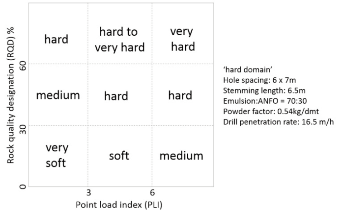
Figure 4. Left: point load index (PLI) versus RQD diagram developed for Batu-Hijau. Use of the diagram allows rocks to be divided into different strength domains each of which requires different drill-and-blast parameters. Right: example of drill-and-blast parameters developed for the ‘hard domain’. ANFO = ammonium nitrate - fuel oil. Modified from Burger et al. (2006).
