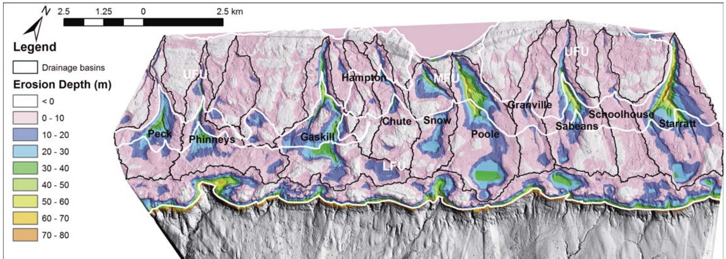
Figure 5. North Mountain drainage basin boundaries (black lines and labels) and erosion depth map with basalt flow unit boundaries (white lines and labels: Lower Flow Unit – LFU, Middle Flow Unit – MFU, Upper Flow Unit - UFU). The western basins have maximum incision depths of approximately 40 m and the central and eastern basins have maximum incision depths approaching 80 m.
