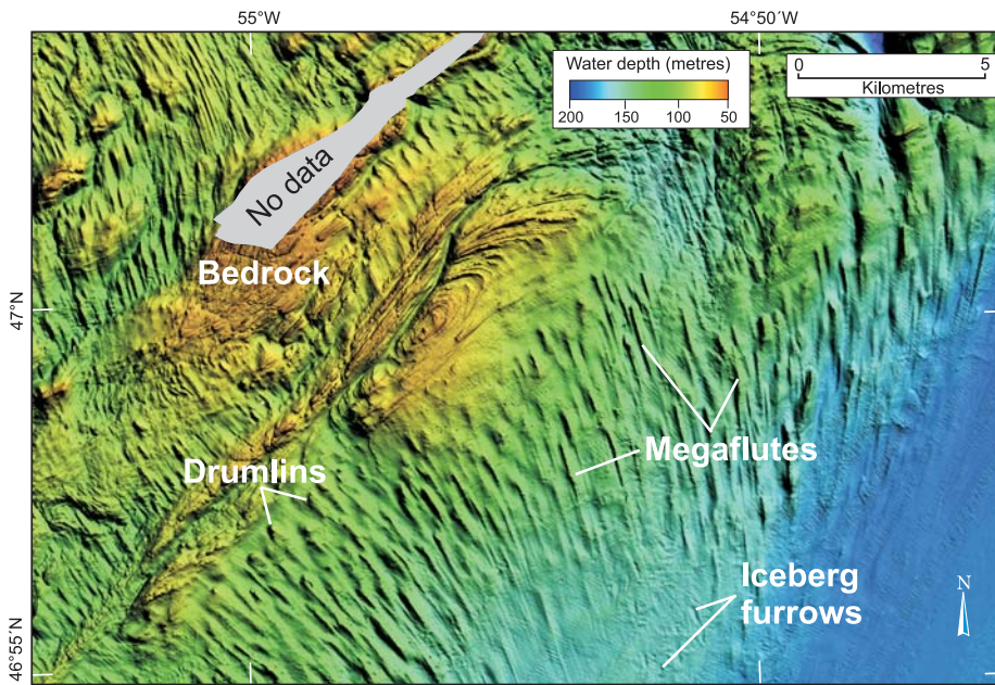
Figure 6. Shaded-relief bathymetry map showing outcropping bedrock mantled by drumlins and megaflutes in Placentia Bay, southern Newfoundland. Drumlins are ridges of ice-contact sediment (till) formed under the ice, and are elongated in the former ice-flow direction. Megaflutes are more elongated than drumlins, and indicate faster ice flow. Here the convergent pattern is indicative of acceleration of grounded ice towards the south. In the bottom right of the image the megaflutes disappear beneath a cover of glaciomarine mud (heavily imprinted by iceberg furrows) and postglacial mud. A more complete description is given in Shaw et al. (2009b).
