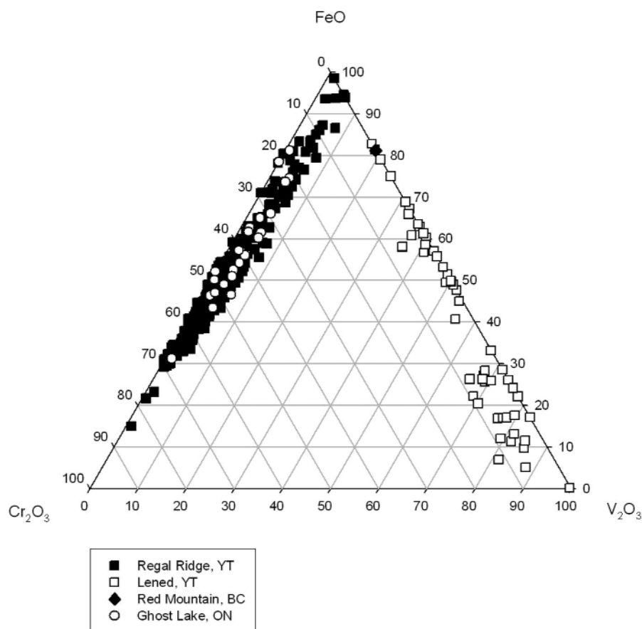
Figure 4. Triangular diagram of \text{Cr}_2\text{O}_3 -FeO- \text{V}_2\text{O}_3 weight percentages from analyses of emerald.
