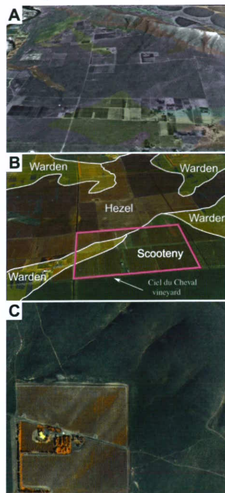
Figure 14 Soil and vegetation patterns for vineyards in the Red Mountain AVA. A) 3-D perspective view of Red Mountain area with soil series draped over black and white ortho aerial photograph. Data from Rasmussen (1971). B) Close-up of 14A showing soil series patterns within individual vineyards. In the Ciel du Cheval vineyard (#5) some vine rows cross three different soil types, providing an opportunity to study the effect of different soil characteristics on grape vine performance with little or no change in climate or viticultural practice. C) Aerial color infrared imagery showing differences in plant vigour relative to topography and soil distribution in the Belle Ville vineyard (#2). Note that in infrared images, green vegetation such as leafy vineyards is red whereas arid range lands are dark green. Images courtesy of Francis Pierce, Center for Precision Agricultural Systems, WSU-IAREC.
