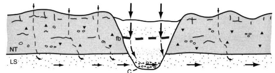
Figure 9 Hydrogeological terrains: (A) thick aquitard setting: Newmarket Till upland; (B) aquitard breach with coarse channel sediment, and (C) aquitard breach with fine-grained sediment beds (fb). Arrows indicate generalized groundwater flux. NT=Newmarket Till; C=channel; LS=lower sediment aquifer.
