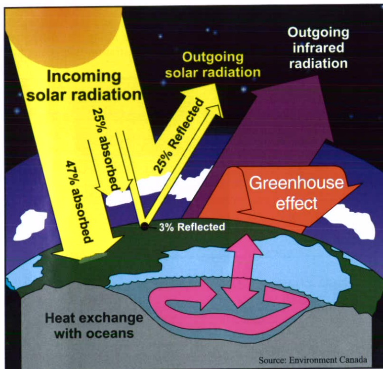
Figure 4 Earth's solar energy budget (Environment Canada, 1993).
