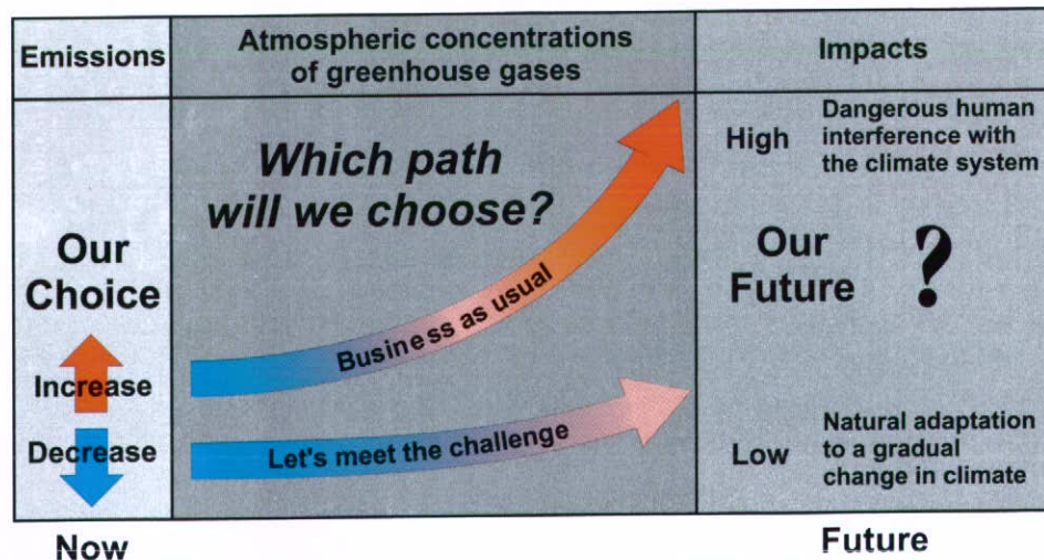
Figure 15 Future consequences of the choice we make today about curtailing greenhouse gas emissions (Turner and Clague, 1999).
