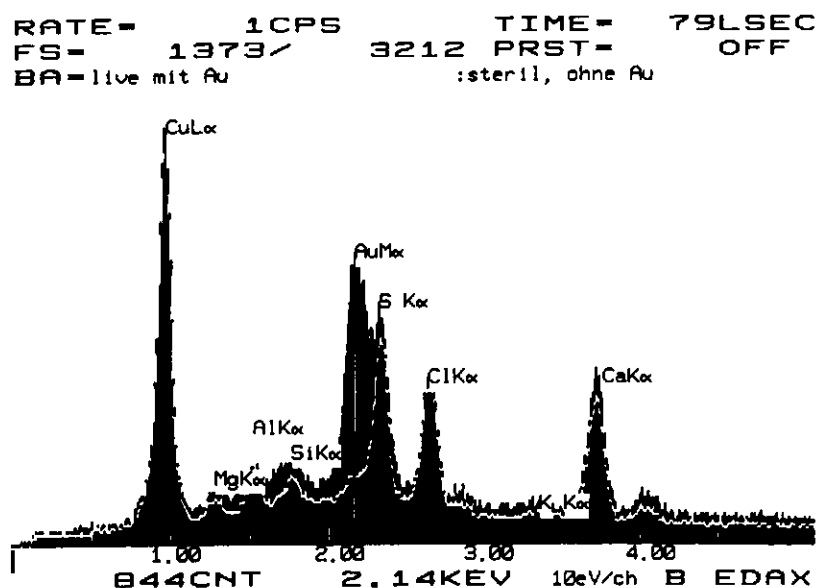
Figure 1 Energy dispersive X-ray microanalysis, at 2.14 KEV, of elements in the glycolyx of a filament of Plectorema terebrans . The solid curve filled in black shows results of analysis of live cultures incubated in gold solution; notice the peak for gold. The superimposed white curve shows results from heat-killed cultures in gold solution. The two curves are similar except for the absence of gold in the heat-killed microorganisms. The analysis was made at a rate of 1 count per second for 79 seconds. (From Dyer et al. , 1994, with permission)
