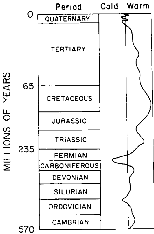
Figure 1 Climatic variability over the Phanerozoic relative to present-day global mean climate. (Modified from Frakes, 1979).
