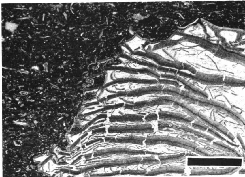
Figure 11 Part of a crushed rugose coral, the victim of physical compaction of the surrounding packstone matrix. Nearshore-marine skeletal limestone from the Mission Canyon Formation (Mississippian), Williston Basin, North Dakota (Beach and Schumacher, 1982a, b). Bar scale is 1 mm. Thin-section loaned by D.K. Beach, photo used by permission.
