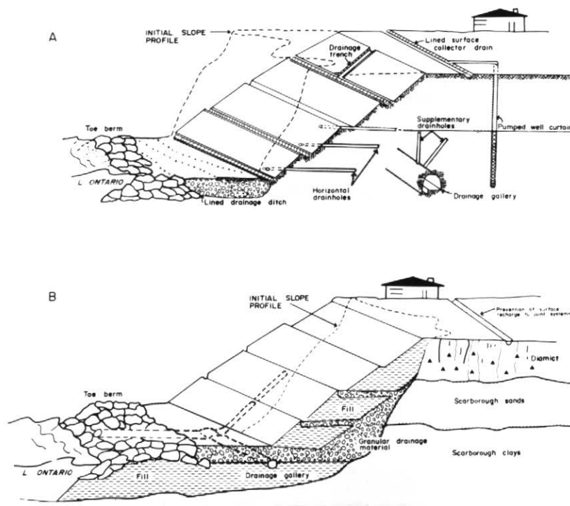
Figure 14 Contrasting slope control and drainage systems. A) Situation where siting of pre-existing structures permits natural or artificial lowering of the bluff slope angle; B) Situation where pre-existing structures are in close proximity to bluff edge and the slope profile has to be lowered by addition of fill. Note toe berms in both cases to prevent the erosion and to buttress lower slope area. After various sources, principally CANMET (1977)
