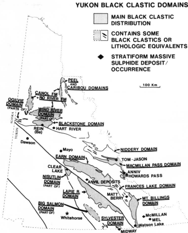
Figure 2 Yukon assessment domains containing Black Clastic and equivalent lithologies.
