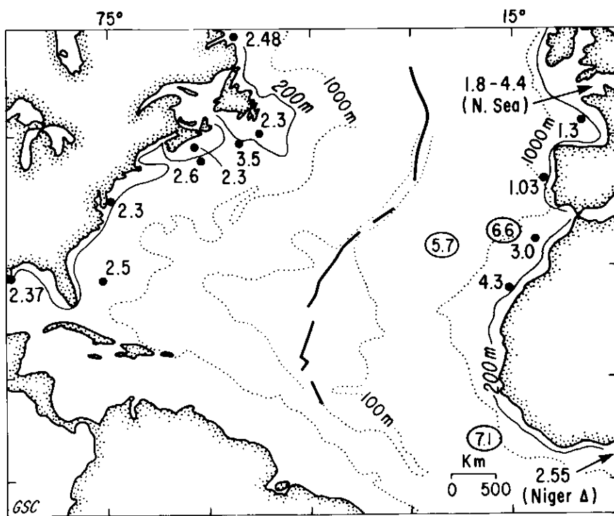
Figure 8 Temperature gradients in the Central North Atlantic Basin. Numbers inside circles represent average geothermal gradient of the region recalculated from Herman et al. (1977).
