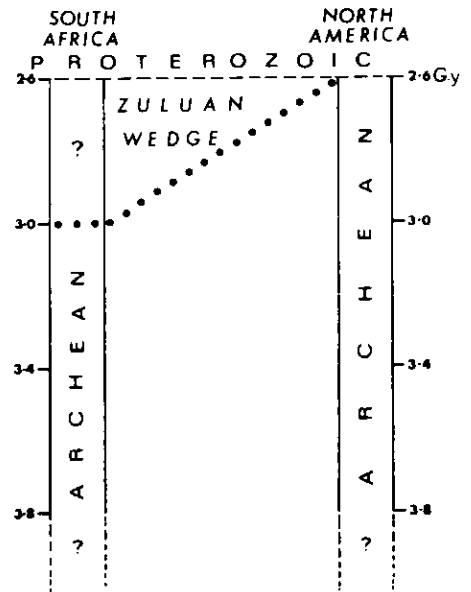
Figure 1 Comparison of some aspects of the Archean-Proterozoic boundary in South Africa (after Cloud, 1976) and in the Canadian Shield (after Stockwell, 1973). The Zuluian Wedge was proposed by Cloud (1976) to accommodate stable shelf-type deposits of the Kaapvaal craton, between 3.0 Ga and 2.6 Ga ago. The figure demonstrates the diachronous development of end-Archean cratonization and some of the problems in establishing the Archean-Proterozoic boundary.
