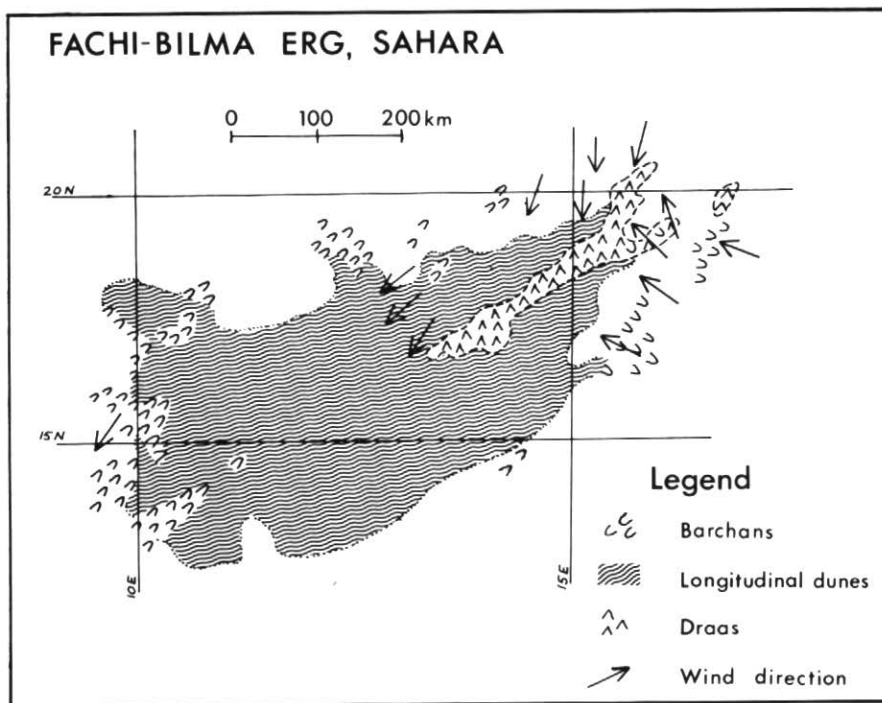
Figure 1 Distribution of dune types and wind directions in the Fachi-Bilma Erg, southeastern Sahara (modified from Mainguet and Callot, 1974).
