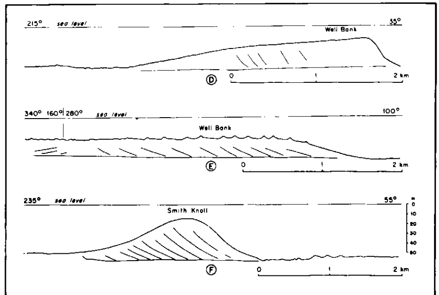
Figure 6 Sparker profiles of tidal sand ridges off southeast England. Although they look like asymmetrical cross-bedded features, compare the vertical and horizontal scales given. Calculated "steep" slopes average only 5 to 6 degrees. (From Houbolt, 1968).
