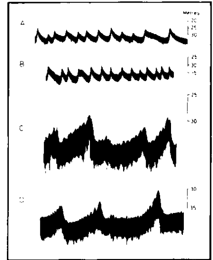
Figure 7 Profiles of sand waves in the southern bight of the North Sea. Vertical scale positioned with respect to sea level = 0 m. Lengths of sections about 3800 m (A); 2800 m (B); 900 m (C); and 1220 m (D); Calculated dips of "steep" faces average 5 degrees. (From McCave, 1971, p 206)
