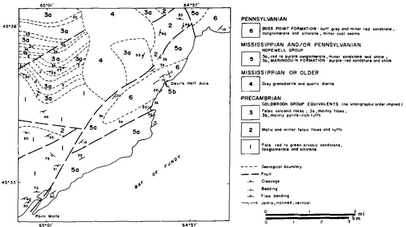
Figure 1 Geological sketch map, Devil's Half Acre area (modified after Kindle, 1958 and Ruitenberg et al., 1975).
