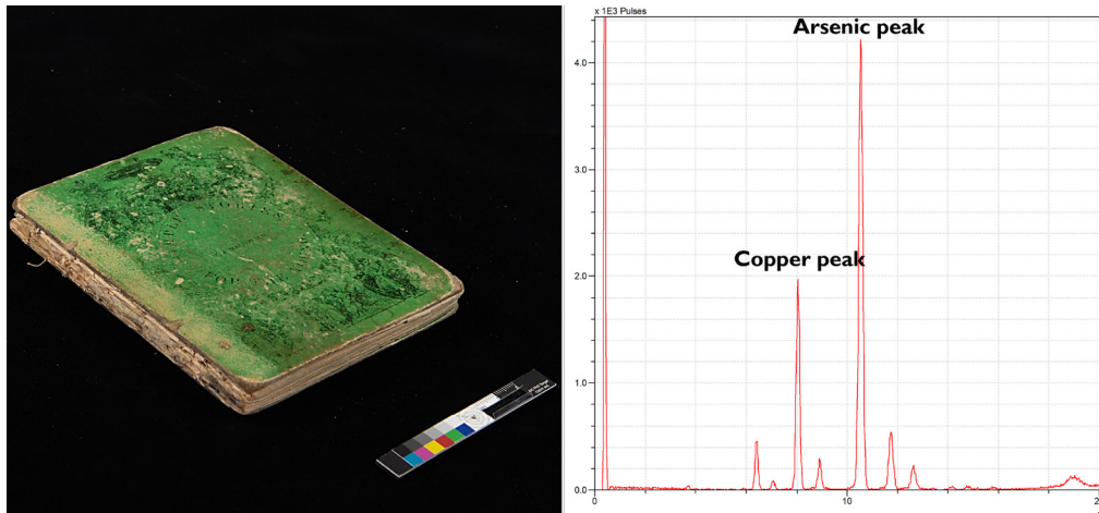
FIGURE 4 (Left) Photograph of the front cover of MacDonal, W.R. Simple Stories for the Amusement and Instruction of Youth , London: Darton & Clark, 1842, Queen's University, Special Collections, Child PZ5 no.1324. (Right) The XRF spectra of the green paper cover demonstrate high peaks for copper and arsenic atoms, as seen in the Bruker ARTAX software. Photo credit: Robin Canham.
