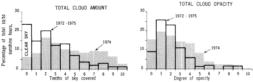
6a. Total amount and opacity for hours of continuous (10/10) bright sunshine: at field observation hours, 1972 - 75, N = 115, solar elevation \geq 24^\circ ; for the growing season, May 16 - October 15, 1974, N = 503, solar elevation \geq 5^\circ .
