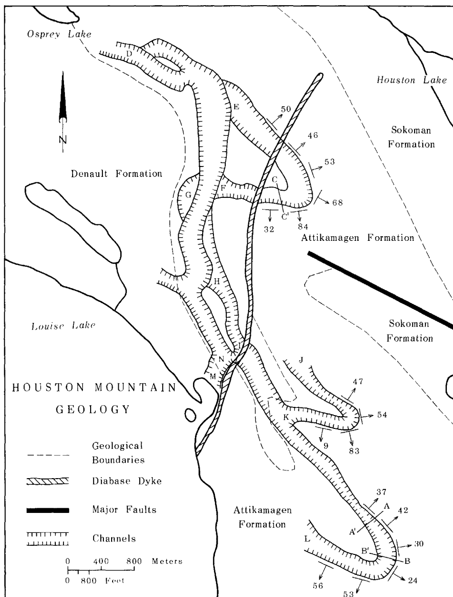
Figure 3 Selected geological features of the Houston Mountain area. Cross-sections A-A', B-B', and C-C 1 are illustrated in Figure 4. Letters locate long-profiles presented in Figure 5.
