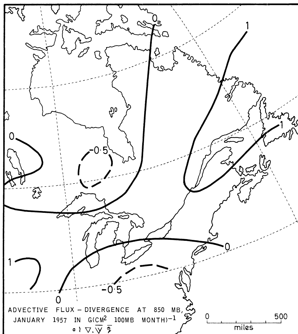
Figure 1a Advective flux-divergence at 850 mb, January 1957 in g \ (cm^2 \ 100 \ mb \ month) (a) \nabla \cdot \overline{\nabla q} (b) \overline{\nabla} \cdot \nabla q
