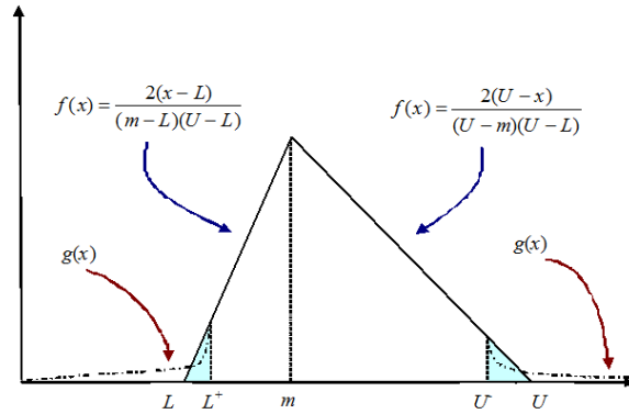
Fig. B.1. Modified Triangular Distribution.
