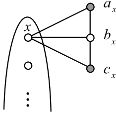
Fig. 6. C is composed of the union of D with all the vertices of the form a_x and c_x in G' .
