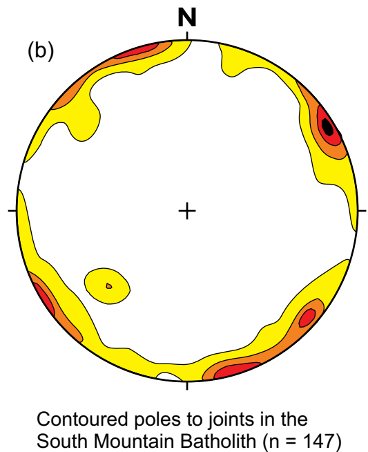
Figure 46. Comparison of jointing in (a) Meguma Supergroup and (b) South Mountain Batholith (after White 2008, with permission). In both stereograms, the darkest shading indicates the highest concentration of poles to the jointing.
