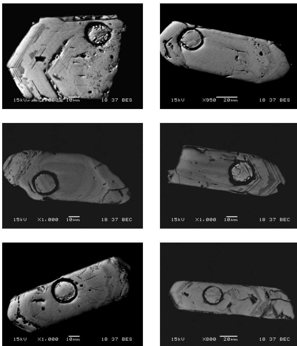
Figure S1. Photomicrographs of representative zircon crystals from the Park Spur pluton taken in back-scattered electron mode showing zoning patterns typical of igneous zircon. Note the different scale bars on the individual images.
